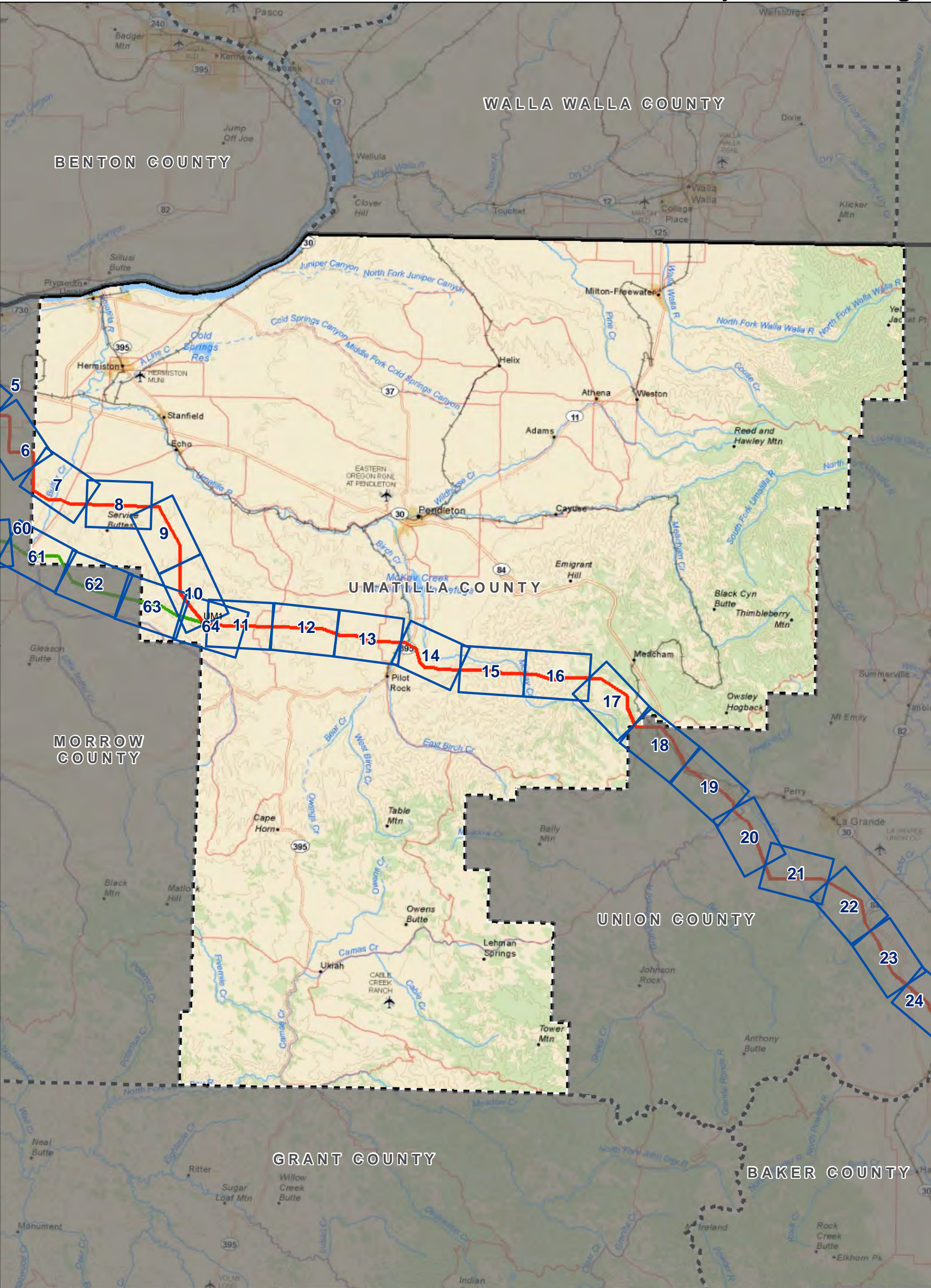
FIGURE 3.1-3 SEGMENT 2 - UMATILLA COUNTY, OR BOARDMAN TO HEMINGWAY 500kV TRANSMISSION LINE PROJECT OREGON-IDAHO
